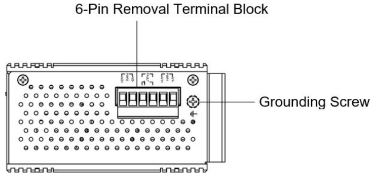
Figure 2.3 - Top View Panel
