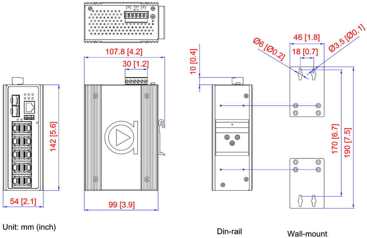
Figure 2.1 - Physical Dimensions
